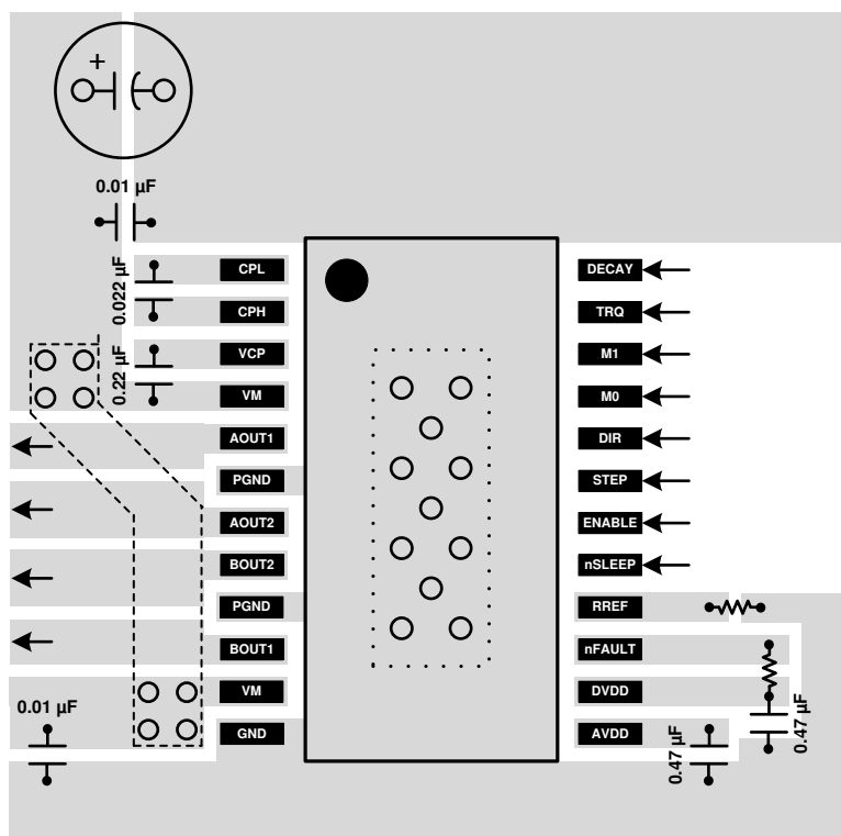
Figure 33. Layout Recommendation
