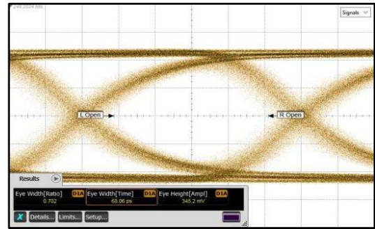
Figure 20. TL = 20 Inch 4-Mil FR4 Trace, DS100BR111A CMA, 10.3125 Gbps
