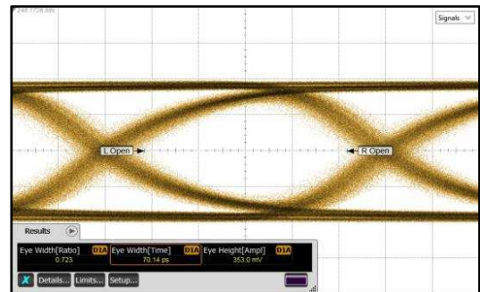
Figure 22. TL = 30 Inch 4-Mil FR4 Trace, DS100BR111A CMA, 10.3125 Gbps
