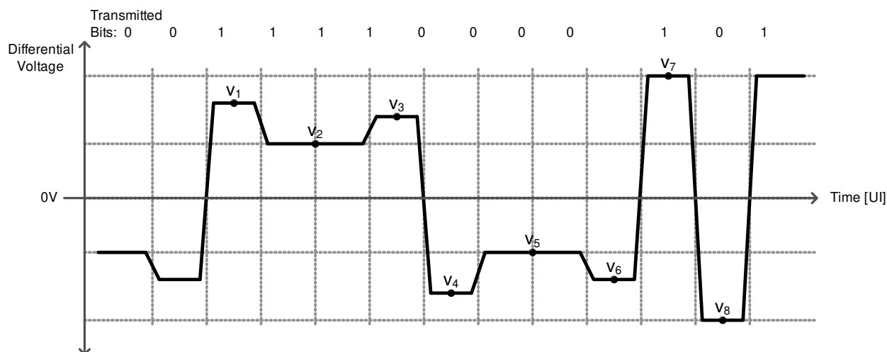
Figure 8-4. Conceptual FIR Waveform With Both Pre- and Post-Cursor
