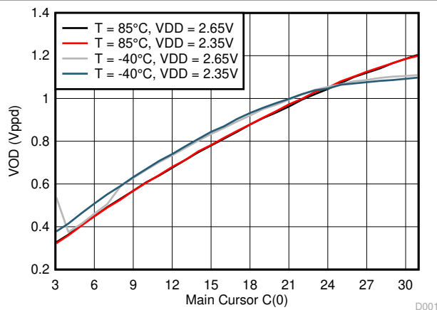
Figure 7-3. Typical VOD vs FIR Main-Cursor
