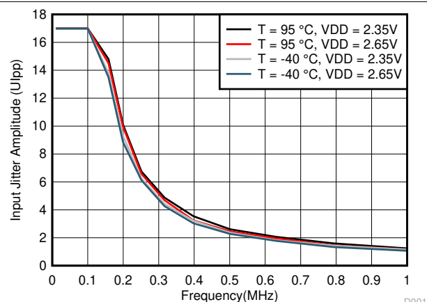
Figure 7-5. Typical Sinusoidal Input Jitter Tolerance for 30-dB Channel at 25.78125 Gbps
