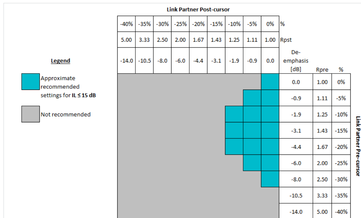
Figure 8-5. Guideline for Link Partner FIR Settings When IL \leq 15 dB
