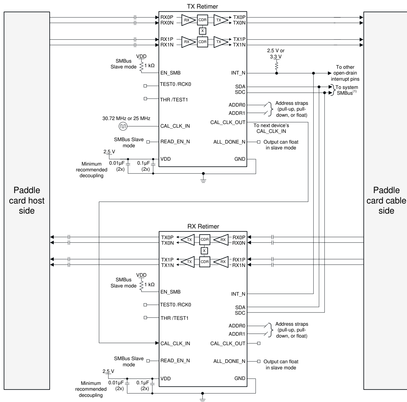
Figure 9-9. Full-Active Cable Application Schematic
