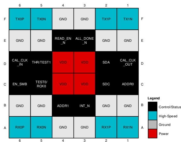
Figure 6-1. ZLS Package 36-Pin NFBGA Top View
