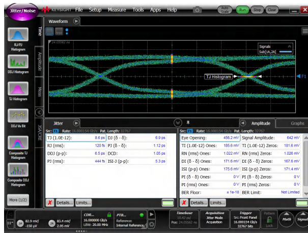
Figure 6-3. Through Baseline Calibration Trace (no redriver) Setup at 16 Gbps
