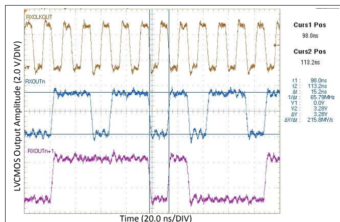
Figure 16. Parallel PRBS-7 on LVC MOS Outputs at 66 MHz
