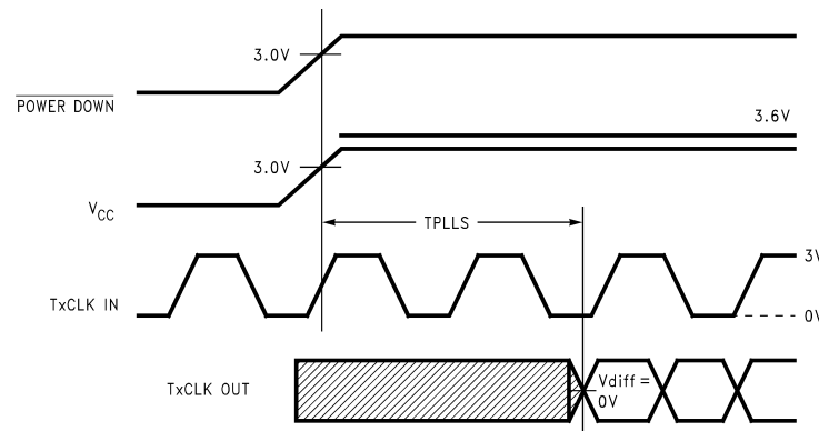
Figure 9. DS90CR483 (Transmitter) Phase Lock Loop Set Time
