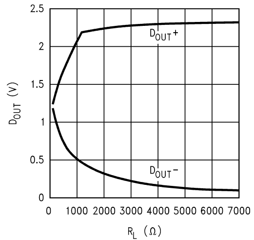
Figure 9. Typical DS90LV031, D O vs R L , V CC = 3.3V, T A = 25°C
