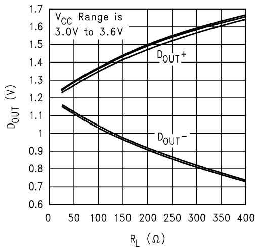
Figure 8. Typical DS90LV031, T A = 25°C D O (single ended) vs R L
