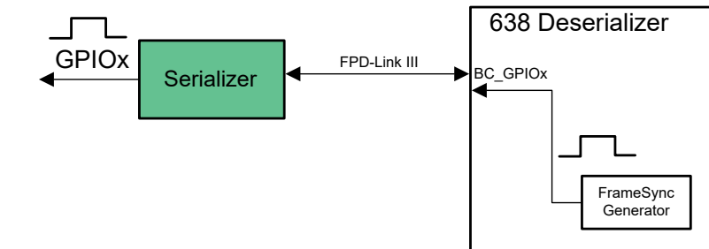
Figure 7-11. Internal FrameSync With DS90UB638 Deserializer
