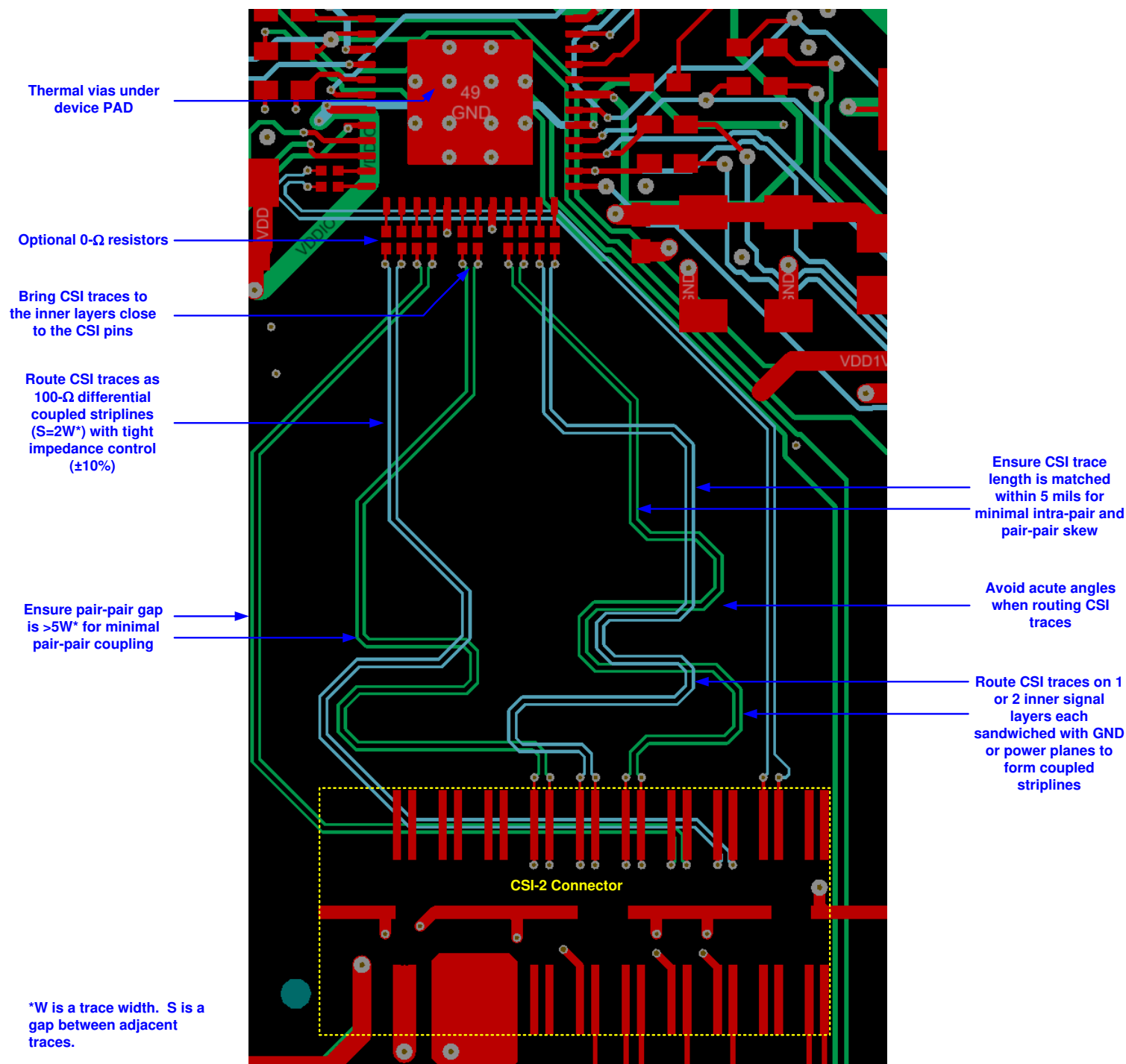
Figure 10-3. DS90UB638-Q1 PCB Layout Example: CSI-2 Traces
