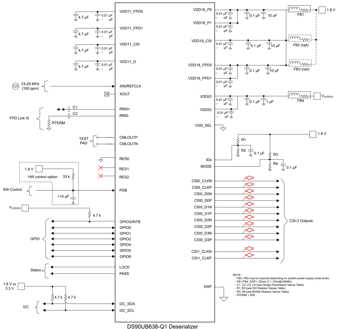
Figure 8-4. Typical Connection Diagram Coaxial With Internal 1.1-V LDO
