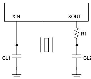
Figure 7-2. Crystal Oscillator Circuit
