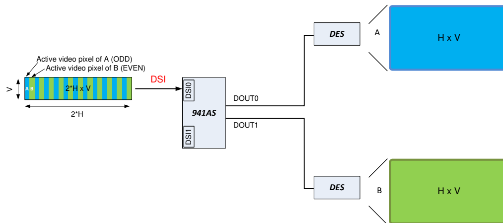
Figure 8-24. Alternate Pixel Splitting
