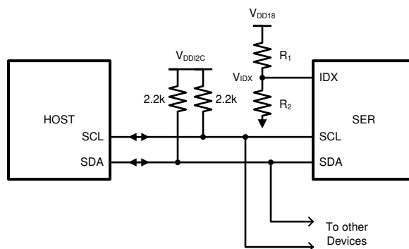
Figure 8-29. Serial Control Bus Connection
