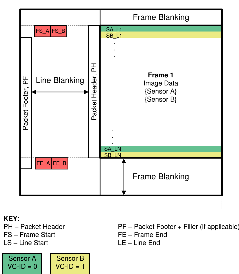
Figure 7-21. Basic Synchronized Format
