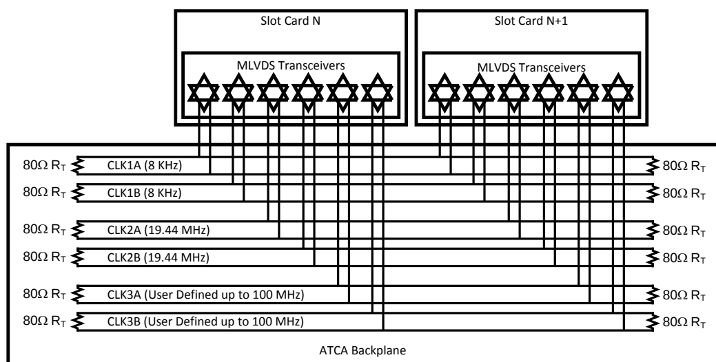
Figure 1. System Diagram
