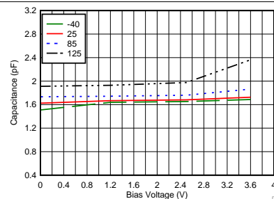
Figure 8. Capacitance Vs. Bias Voltage at Different Temperatures ( ^{\circ} C)
