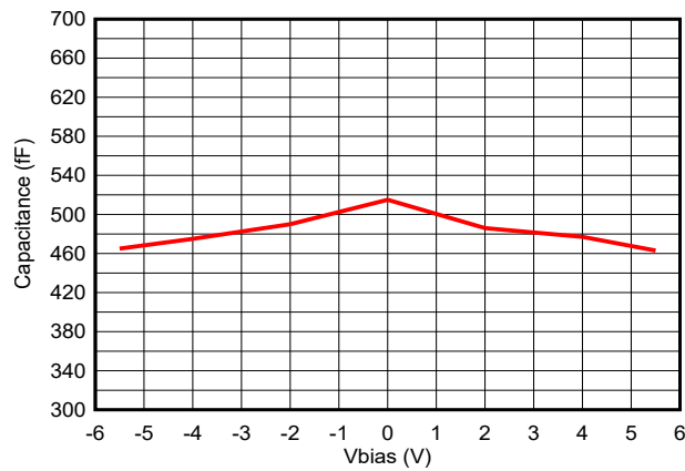
Figure 5-13. Bias Voltage vs. Capacitance (DPY)
