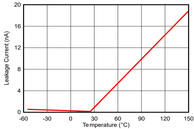
Figure 5-7. Leakage Current vs Temperature (DXA)
