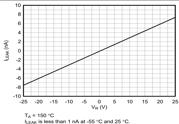
Figure 5-14. Leakage Current vs. Bias Voltage Across Temperature (DBZ/DCK)
