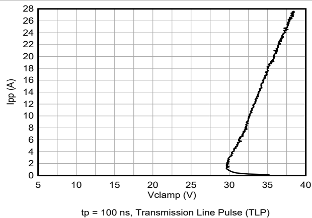
Figure 5-11. Positive TLP Curve (DBZ/DCK)
