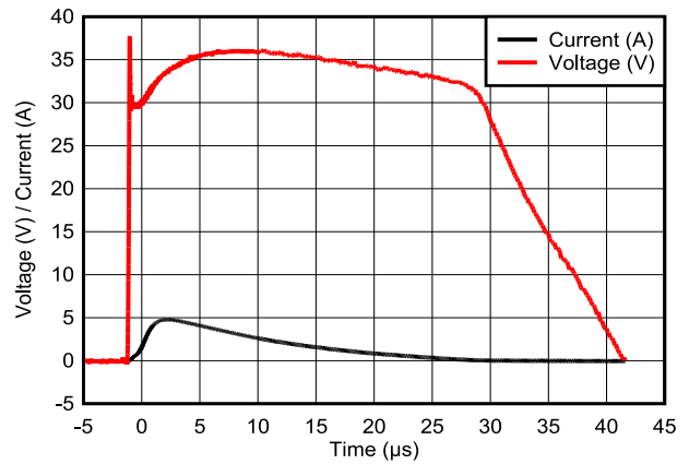
Figure 5-8. 8/20µs Surge Response (DXA)
