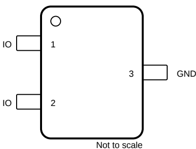
Figure 4-2. DBZ & DCK Package, 3-Pin SOT-23 & SOT SC70 (Top View)
