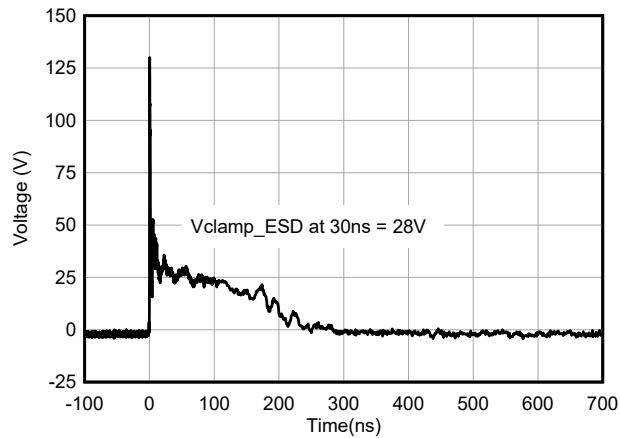
Figure 5-9. +8kV Clamped IEC Waveform (DBZ/DCK)
