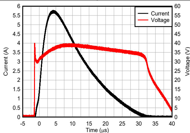
Figure 5-15. 8/20 \mu s Surge Response (DBZ/DCK)
