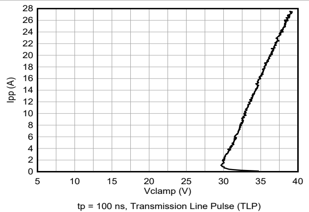
Figure 5-12. Negative TLP Curve (DBZ/DCK)
