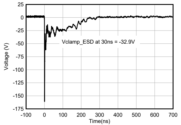
Figure 5-10. -8kV Clamped IEC Waveform (DBZ/DCK)
