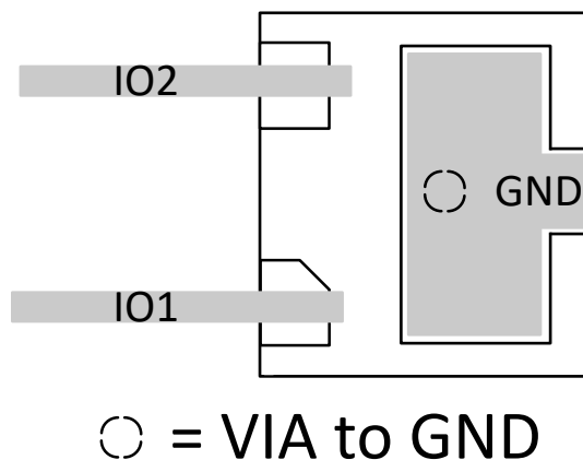
Figure 7-1. Routing with DXA Package
