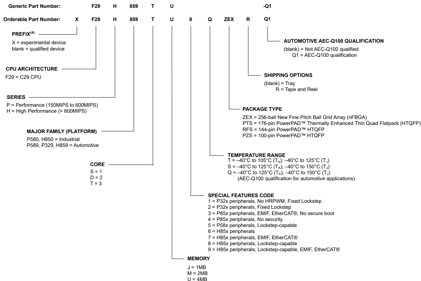
Figure 9-1. Device Nomenclature
