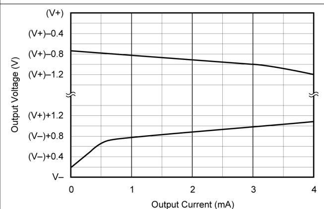
Figure 5-18. Output Voltage Swing vs Output Current
