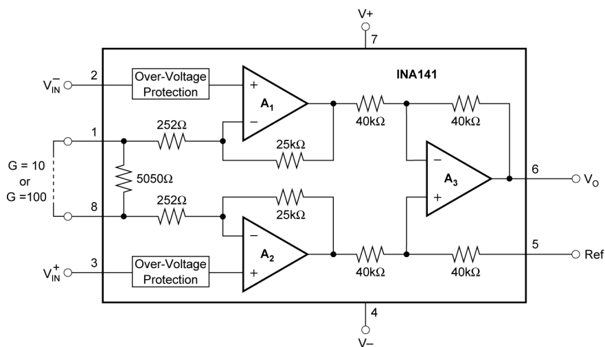
Basic Connections
