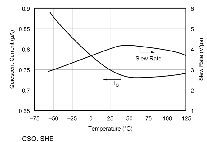
Figure 5-13. Quiescent Current and Slew Rate vs Temperature
