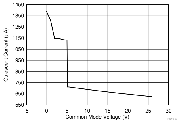
Figure 7-28. Quiescent Current vs. Common-Mode Voltage for All Amplifiers (INA4180-Q1)
