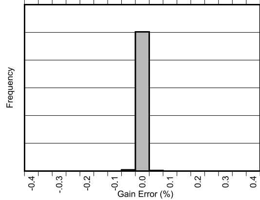
Figure 7-8. Gain Error Production Distribution (A2 Devices)
