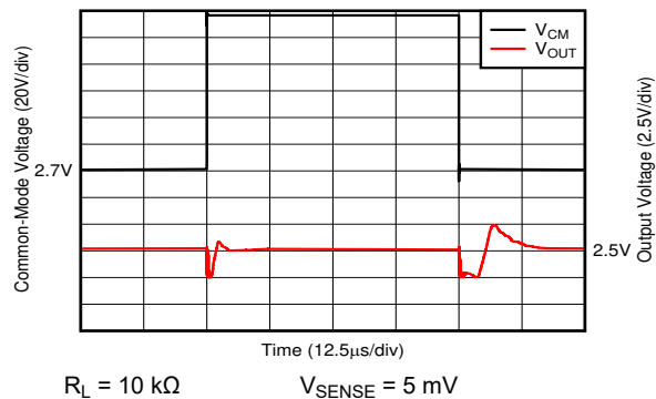
Figure 6-40. Common-Mode Voltage Fast Transient Pulse, A5 Devices
