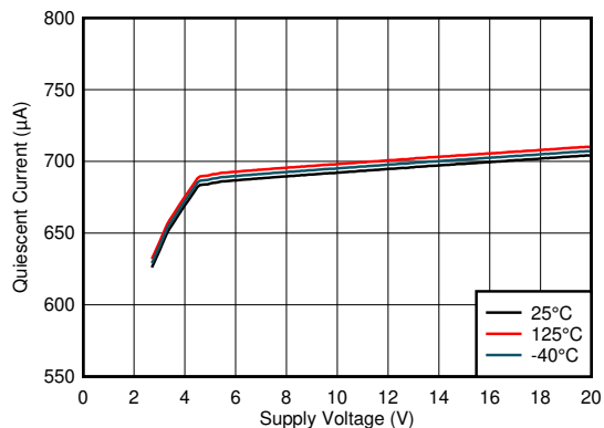
Figure 6-35. Quiescent Current vs. Supply Voltage, INA2290
