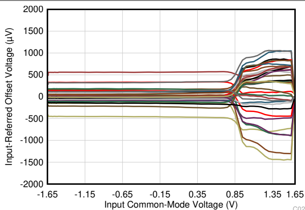
Figure 7-17. Input Referred Offset Voltage vs Input Common-Mode Voltage
