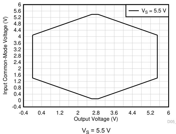
Figure 7-47. Input Common-Mode Voltage vs Output Voltage (High CMRR Region)
