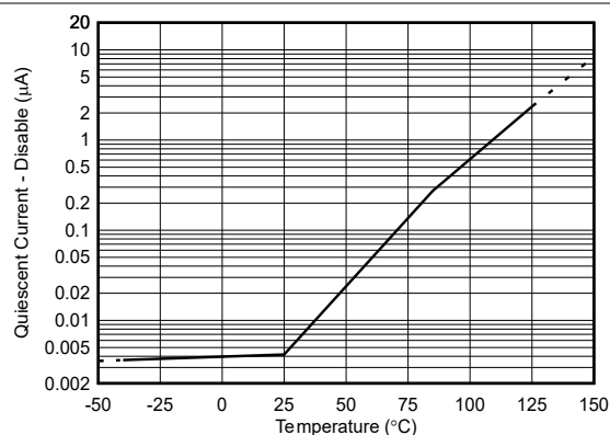
Figure 5-21. Quiescent Current - Disabled vs. Temperature
