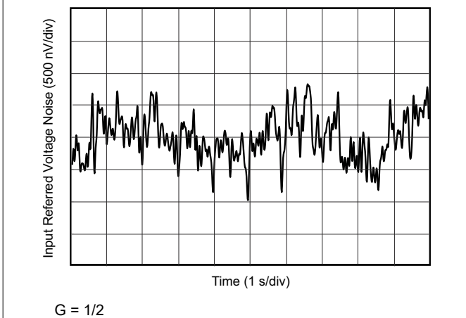
Figure 7-35. 0.1-Hz to 10-Hz RTI Voltage Noise
