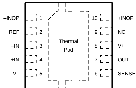
Figure 6-2. DRC (10-Pin VSON With Thermal Pad) Package, Top View
