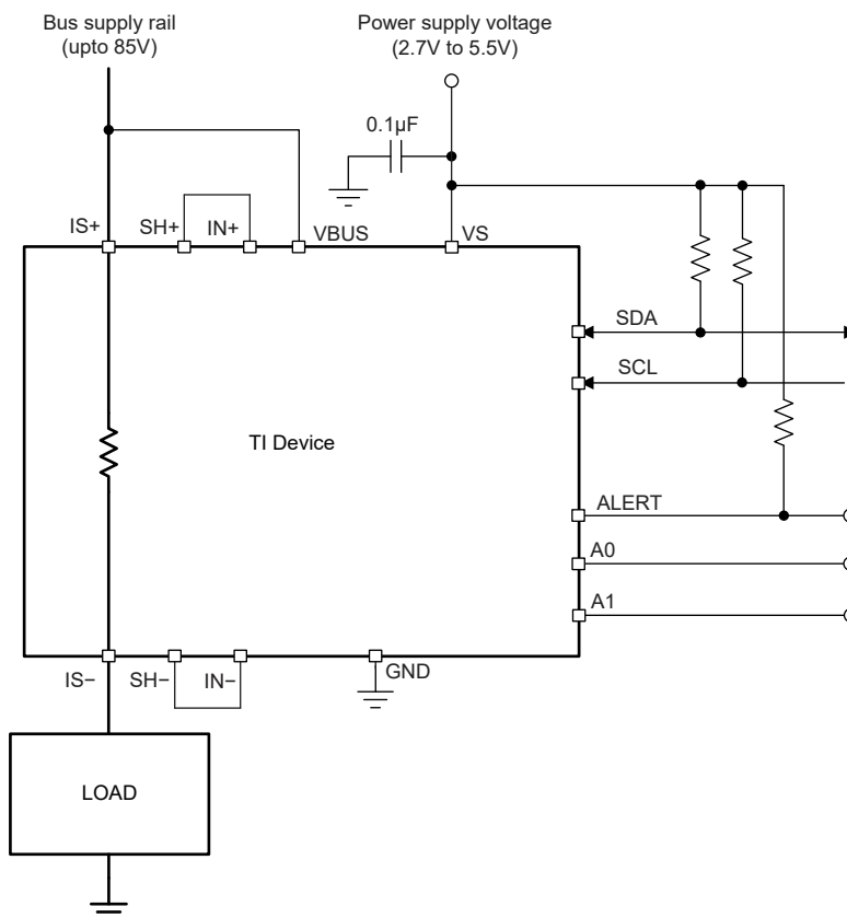
Figure 8-2. INA740B High-Side Sensing Application Diagram
