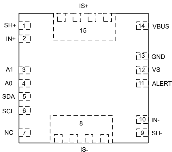
Figure 5-1. DEK Package 15-Pin WSON Top View
