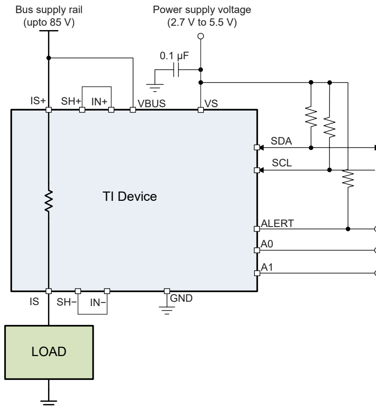
Figure 8-2. INA781 High-Side Sensing Application Diagram
