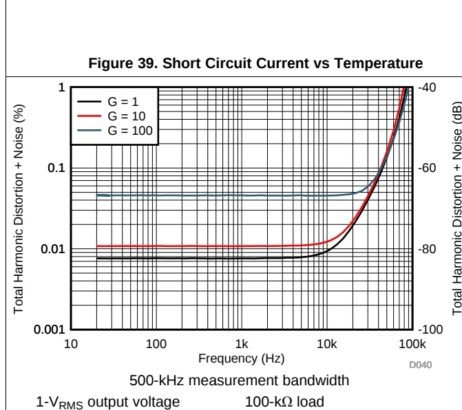
Figure 41. THD+N vs Frequency
