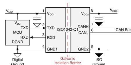
Application Diagram
