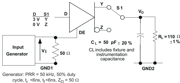
Figure 7-5. Driver High-Level Output Enable and Disable Time Test Circuit and Voltage Waveforms
