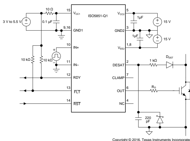
Figure 44. Bipolar Output Supply
