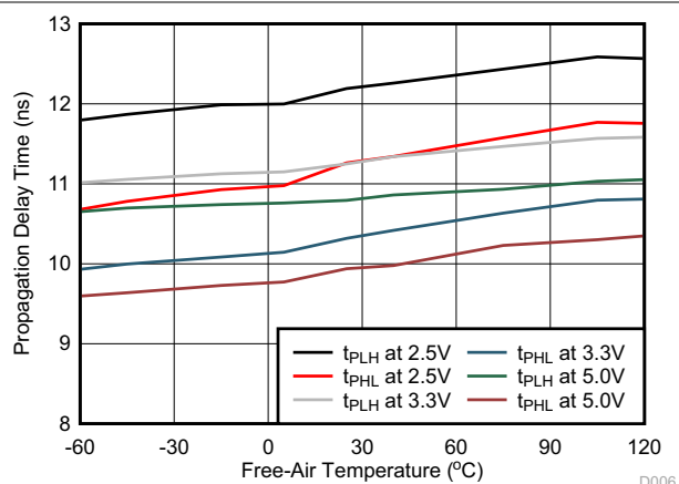
Figure 5-12. Propagation Delay Time vs Free-Air Temperature
