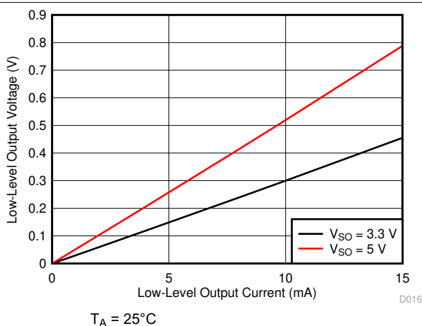
Figure 7-24. Low-Level Output Voltage vs Low-Level Output Current
