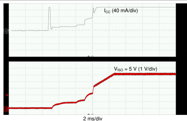
Figure 7-27. Soft Start at 120-mA Load
