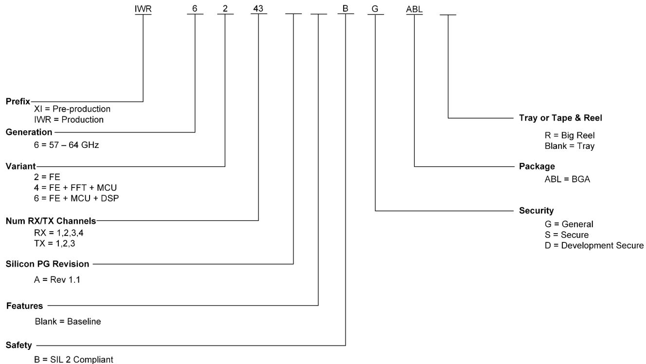
Figure 12-1. Device Nomenclature
