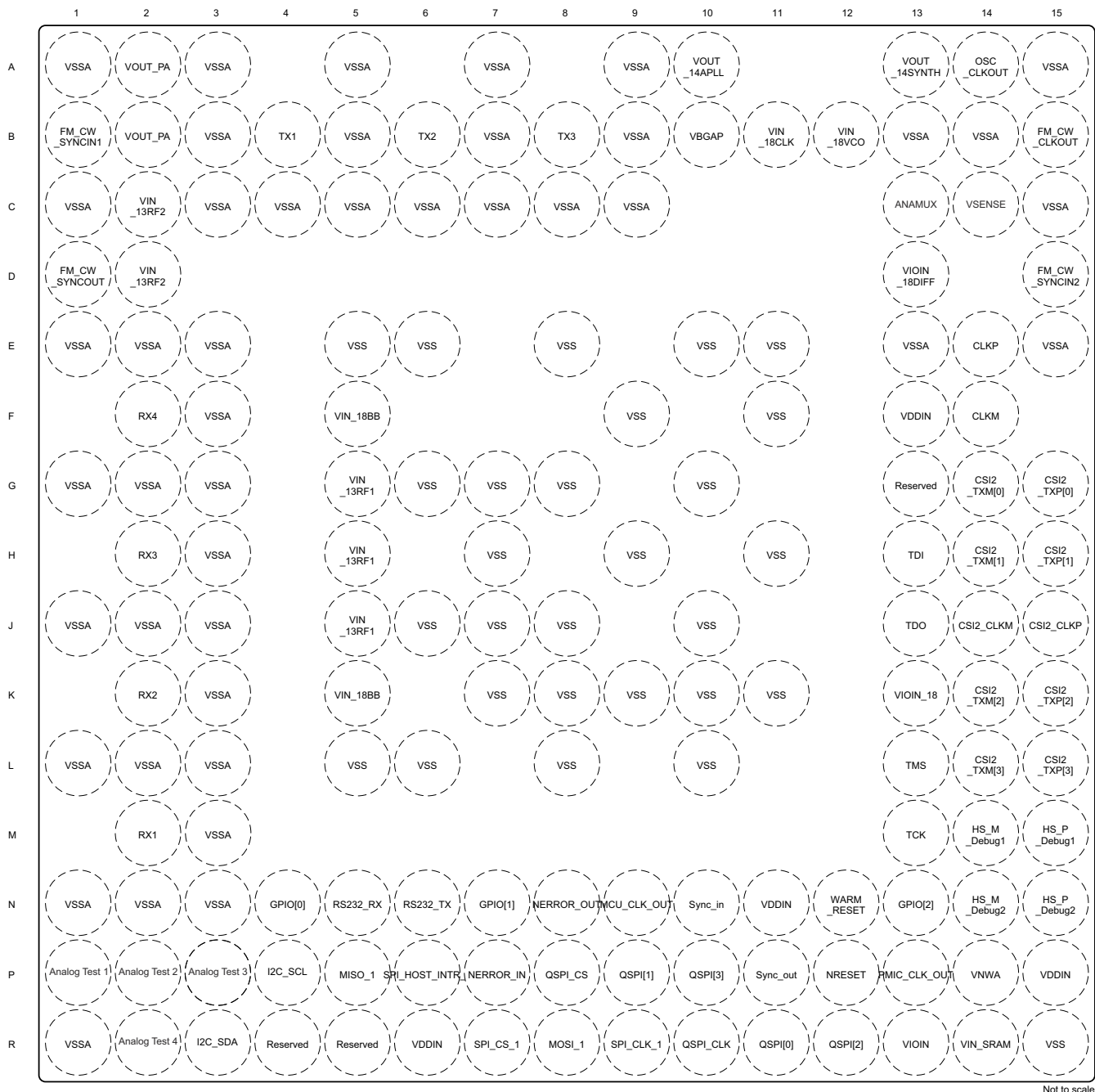
Figure 7-1. Pin Diagram
