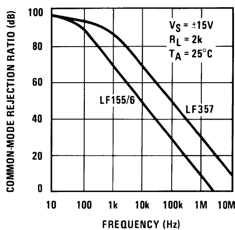
Figure 28. Common-Mode Rejection Ratio
