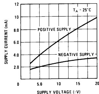
Figure 22. Supply Current
