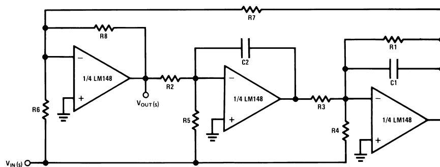
Figure 24. A 1 kHz 4 Pole Butterworth
