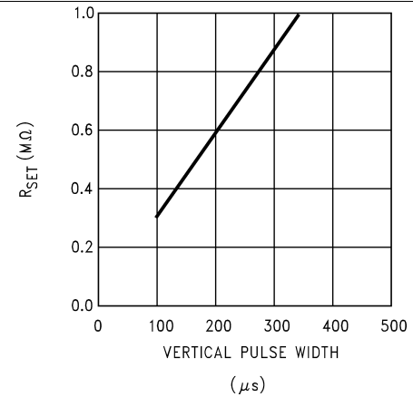
Figure 4. Vertical Pulse Width vs R_{SET}
