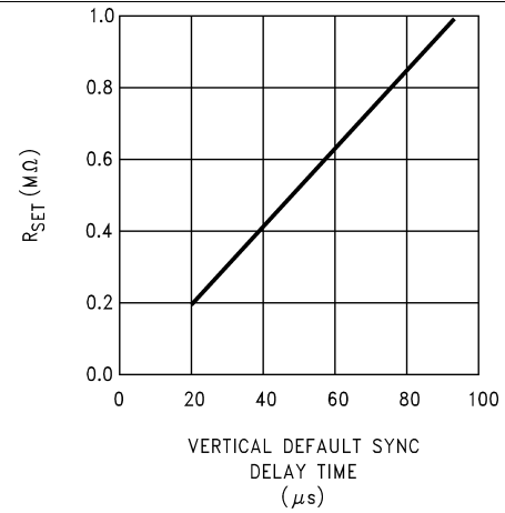
Figure 2. Vertical Default Sync Delay Time vs R_{SET}
