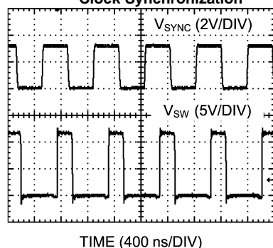
Clock Synchronization
