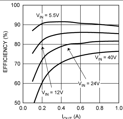
Figure 15. Efficiency vs I_{OUT} and V_{IN} , V_{OUT} = 3.3 \text{ V}
