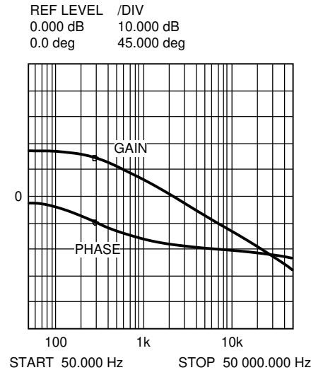
Figure 7-4. Gain and Phase of Modulator R_{\text{LOAD}} = 5\Omega and C_{\text{OUT}} = 177\mu\text{F}
