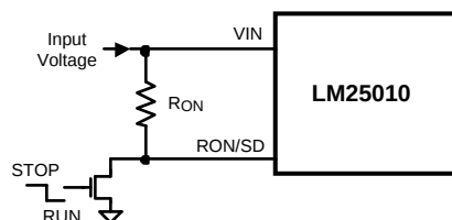
Figure 10. Shutdown Implementation
