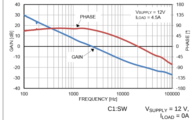
Figure 46. Loop Response
