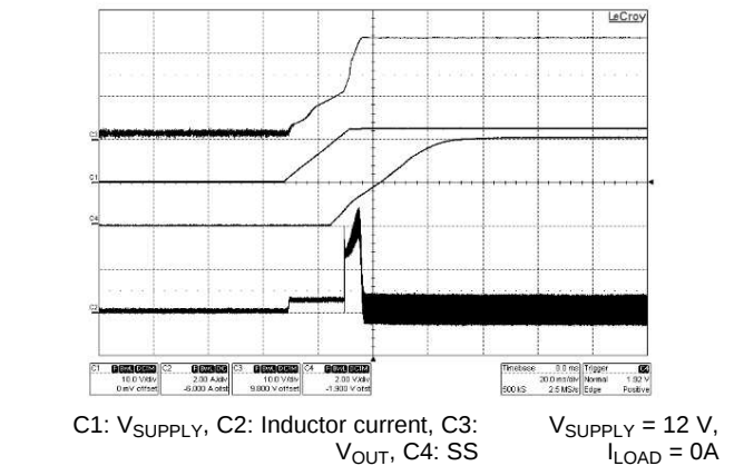
Figure 47. Start-Up
