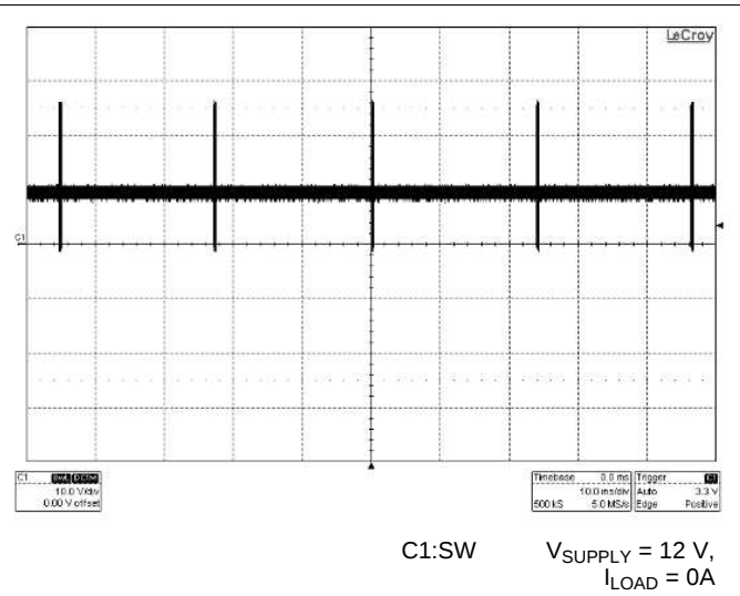
Figure 45. Skip Cycle
