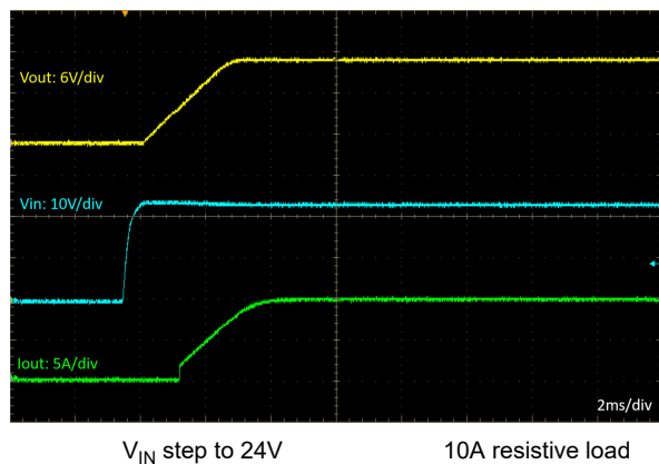
Figure 7-9. Start-Up Characteristic
