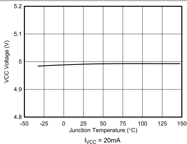
Figure 5-15. VCC Regulation Voltage vs Temperature
