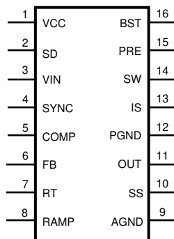
Figure 4-1. PWP 16-Lead HTSSOP (Top View)
