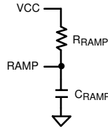
Figure 6-3. R_{RAMP} to V_{CC} for V_{OUT} > 7.5V
