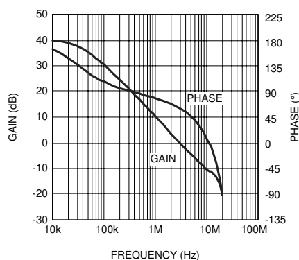
Figure 5-5. Error Amplifier Gain and Phase
