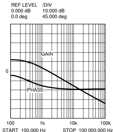
Figure 7-4. Gain and Phase of Modulator R_{LOAD} = 5 \text{ Ohms} and C_{OUT} = 130 \mu\text{F}
