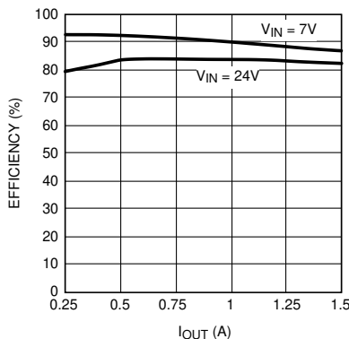
Figure 7-7. Demoboard Efficiency Vs I_{OUT} and V_{IN}
