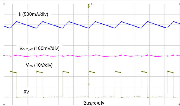
Figure 7-9. Steady State Waveform
