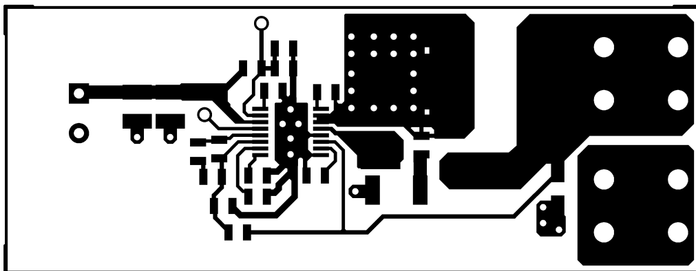
Figure 7-11. Component Side
