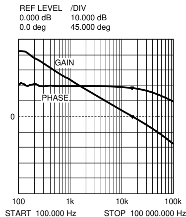
Figure 7-8. Overall Loop Gain and Phase
