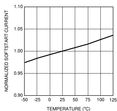
Figure 5-2. Soft Start Current vs Temperature
