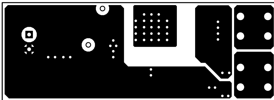
Figure 7-12. Solder Side
