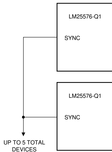
Figure 6-3. Sync from External Clock
