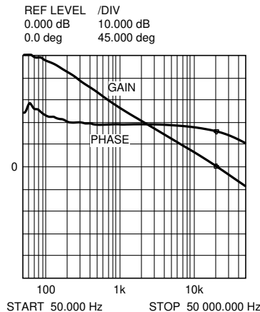
Figure 7-4. Overall Loop Gain and Phase
