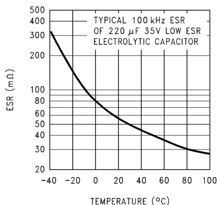
Figure 9-3. Capacitor ESR Change versus Temperature
