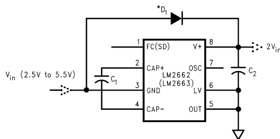
Figure 27. Positive Voltage Doubler
