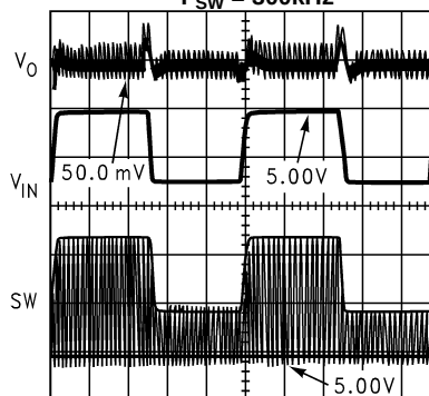
400 \mu s/DIV Figure 23.
