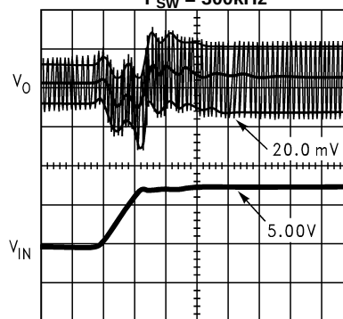
40 \mu s/DIV Figure 21.
