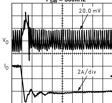
20 \mu s/DIV Figure 20.
