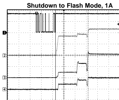
CH1: SDA; Scale: 2V/Div, DC Coupled CH2: V_{OUT} ; Scale: 2V/Div, DC Coupled CH3: I_{IN} ; Scale: 1A/Div, DC Coupled CH4: I_{LED} ; Scale: 1A/Div, DC Coupled Time scale: 1ms/Div
