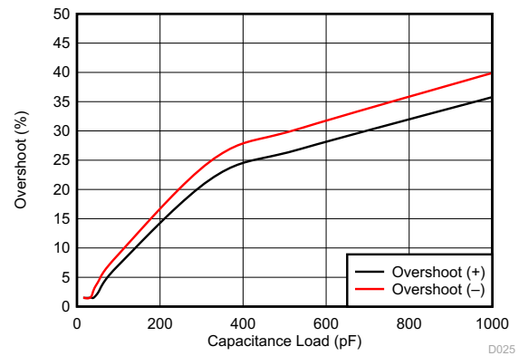
G = -1 V_{IN} = 100\text{ mVpp} Figure 6-19. Small Signal Overshoot vs Capacitive Load
