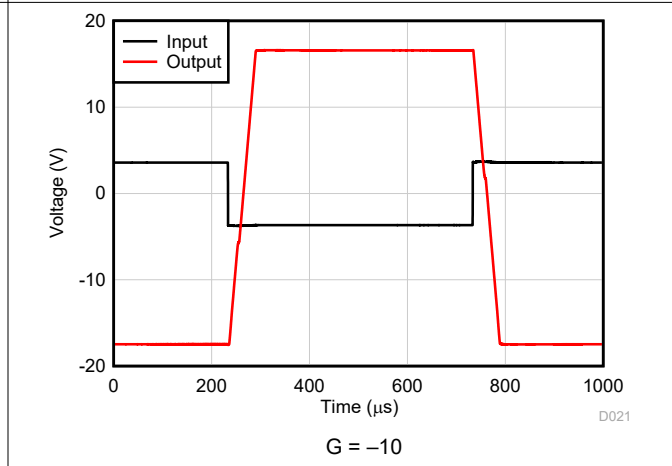
Figure 7-28. Overload Recovery
